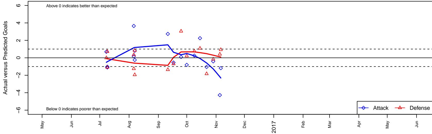
Breakers Red Bryant B99 Dots are actual minus expected GF (blue circles) and GA (red triangles). Blue line is smoothed change in attack strength. Red is smoothed change in defense strength.
